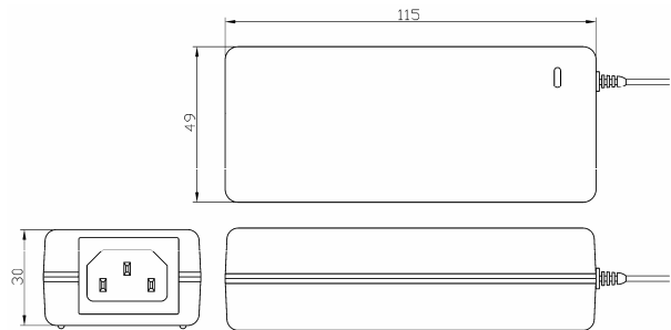
Mechanical Drawing:
